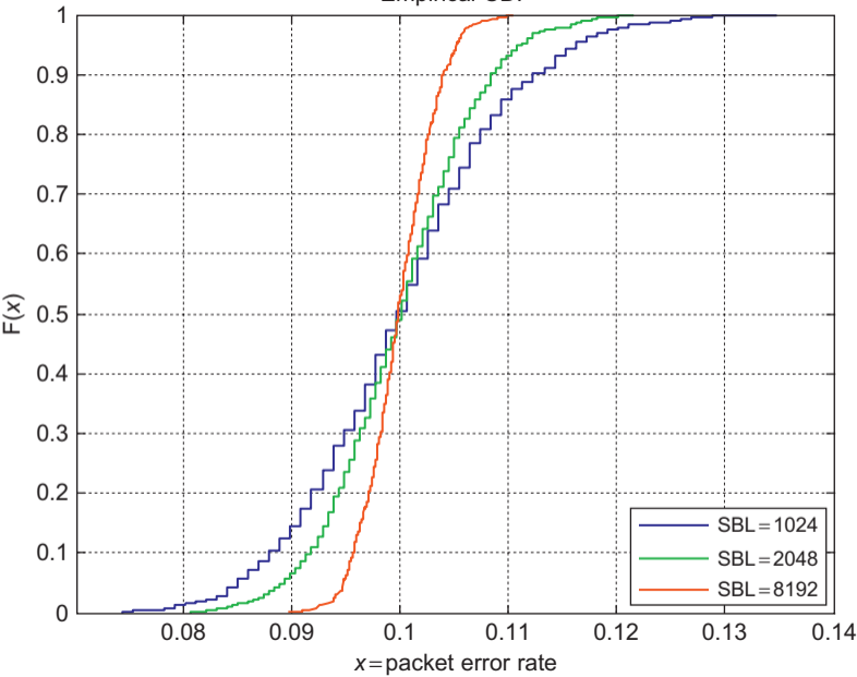
Empirical CDF
