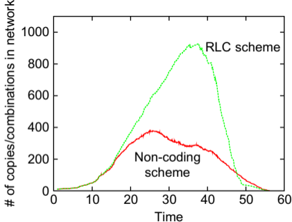
(b) Storage consumption under one run
