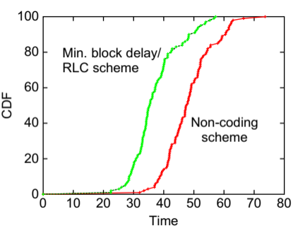
(a) CDF of block delivery delay, 100 runs
