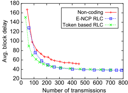
(b) Delay vs number of transmission trade-off ( b=1, B=2 )
