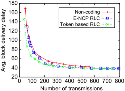
(a) Delay vs number of transmission trade-off ( b=1, B=\infty )
