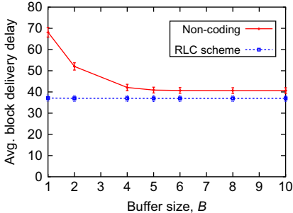
(b) E[D_{block}] under varying buffer
