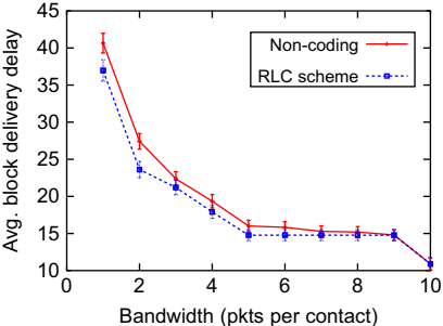
(a) E[D_{block}] under varying bandwidth
