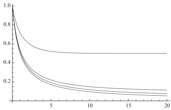
FIGURE A.2 The effects of changing the carrying capacity on solutions of the logistic equation
