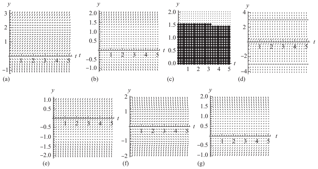
FIGURE A.1 Using direction fields to investigate stability
