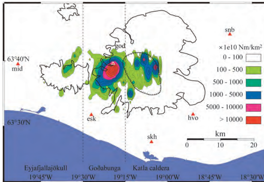
Fig. 2.7. Earthquake activity recorded from 1 January, 1997, to 1 January, 2008, in Eyjafjallajökull and Katla. Contours depict the cumulative seismic moment per square kilometre for the period. Seismic moment was calculated using the moment-magnitude relation \log M_0 = 1.5M_{LW} + 9.1 . Earthquake activity is focused in three regions, separated by dashed lines: two in the Katla volcano; the area within the Katla caldera (2,176 events) and the Goðabunga region (11,951 events), separated by the dashed line, and in Eyjafjallajökull (396 events). Triangles mark locations of seismic stations of the national network, called with the acronym SIL.
